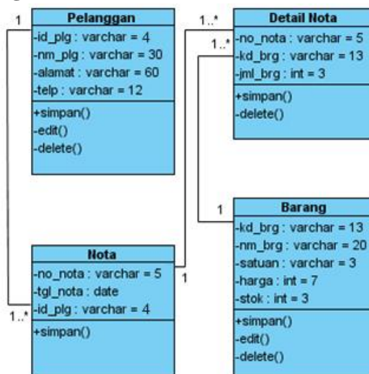
Gambar 4. Class Diagram
