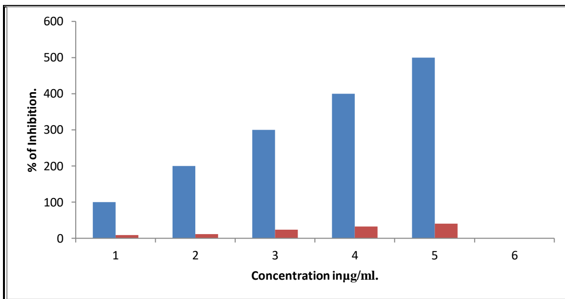
Fig. 2: shows the free radical scavenging activity of chloroform extract of Muntingia calabura .
