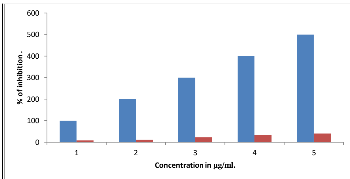
Fig. 1: shows the radical scavenging activity of BHT
