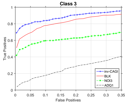
Figure 10: ROC curves in the Fontani et al. synthetic dataset Class 3: inv-CAGI, BLK, NOI3, ADQ1.
