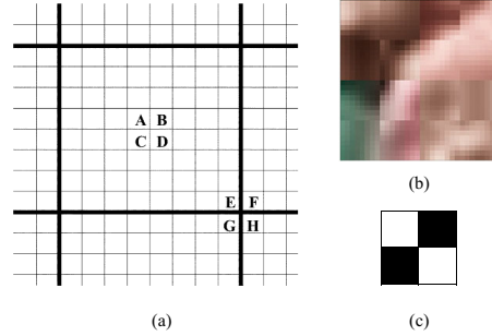
Figure 2: a) Depiction of JPEG 8 \times 8 grid (bold lines) over image pixels. Pixels labeled A-D are sampled periodically to represent the inner part of the grid, while E-H are sampled on grid intersections [3], b) 32 \times 32 JPEG image displaying visible grid artifacts, c) Pixel intensity pattern (cross pattern) maximizing Z' and Z'' (Equation 1).
