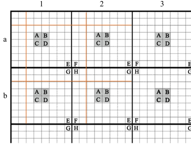
Figure 5: Example of multiple JPEG grids. Black grid is the original grid and orange grid is introduced by a tampering operation, e.g. splicing.
