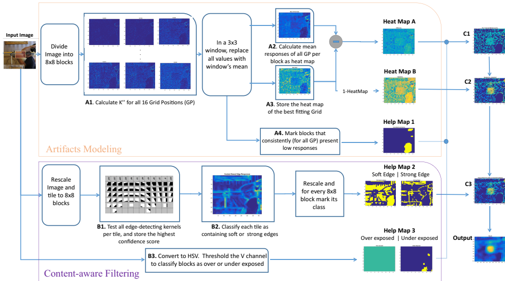
Figure 6: Overview of the proposed method with visualized example results of the intermediate stages and final output.
