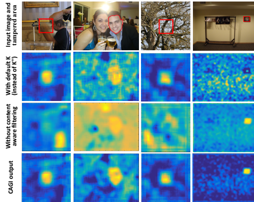
Figure 1: Examples showcasing the contributions of CAGI. First row : input images where the tampered area is marked with a red outline. Second row : Outputs maps produced without the newly proposed grid alignment confidence measure. Third row : Output maps produced without the content-aware filtering step. Fourth row : Output maps produced by the CAGI method.
