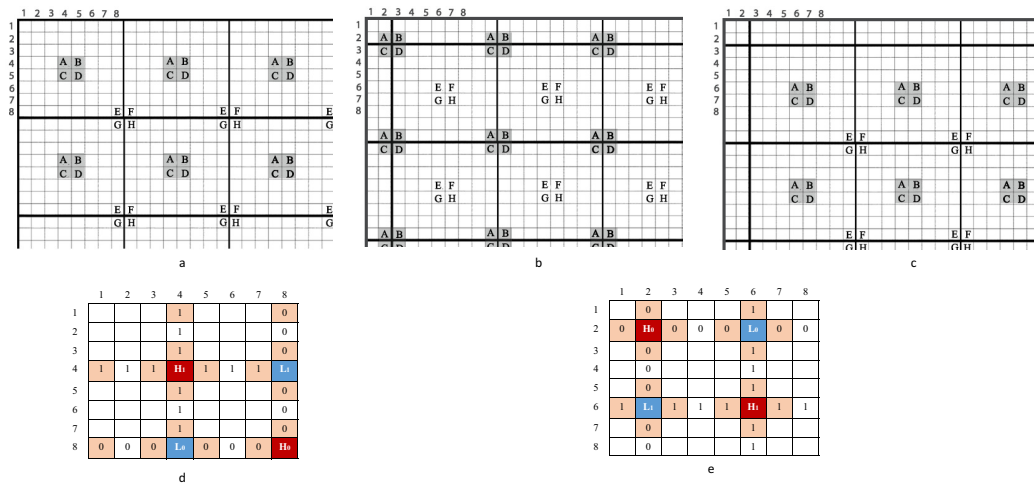
Figure 4: Visualized bitmap examples of grids at position a) GP(4,4) , and b,c) GP(6,6) , with marked sampling instances that present the highest K scores. Expected K -score patterns for d) GP(4,4) , and e) GP(6,6) .
