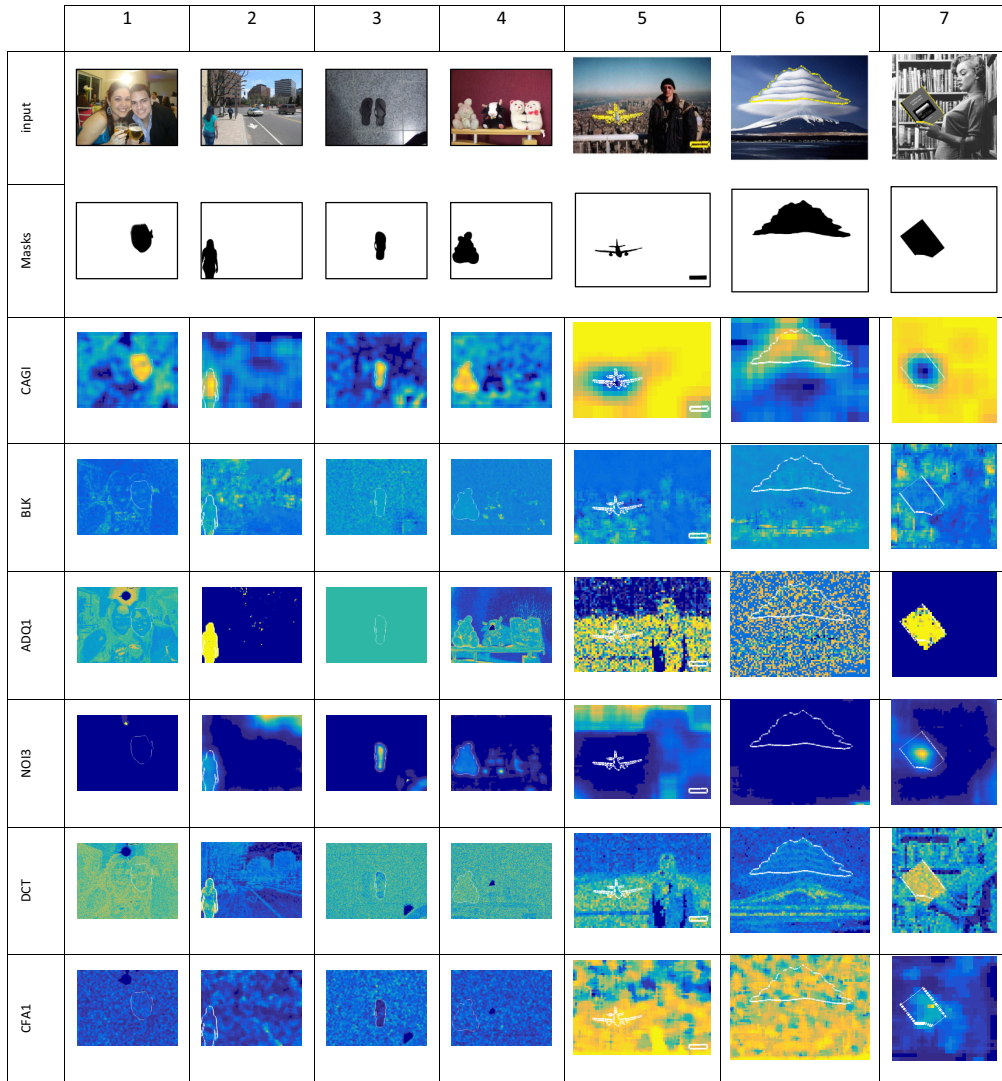
Figure 14: Heat maps produced by the methods: Input images in columns 1-4 are taken from the Challenge dataset and columns 5-7 from the Wild Web dataset. For the proposed method, the outputs shown for input images 1-4 and 6 are produced by CAGI, while for images 5 and 7 they were produced by inv-CAGI. The tampered part in each case is drawn using a white outline on all heat maps.
