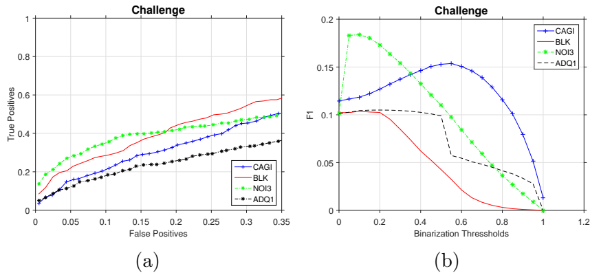
Figure 11: Results on the Challenge dataset: a) ROC curves, b) F1 score curves.
