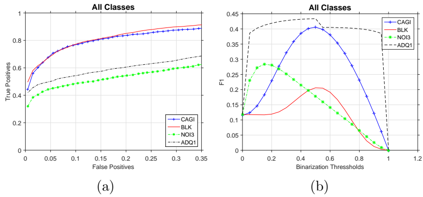
Figure 8: Results in the Fontani et al. synthetic dataset over all classes: a) ROC curves, b) F1 score curves.
