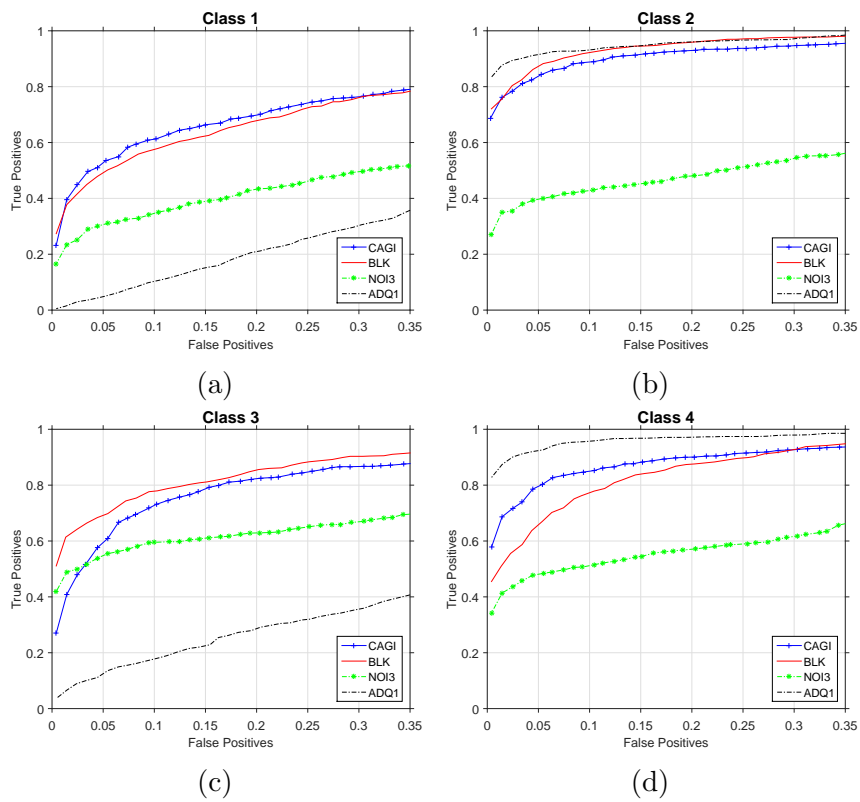
Figure 9: ROC curves in the Fontani et al. synthetic dataset per class: a) Class 1, b) Class 2, c) Class 3, d) Class 4.
