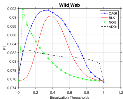
Figure 12: F1 score curves on the Wild Web dataset.
