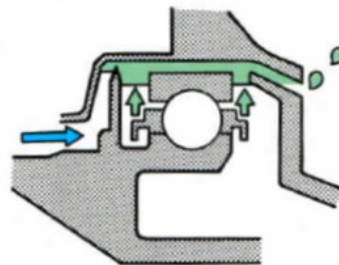
THREAD TYPE (labyrinth) OIL SEAL
