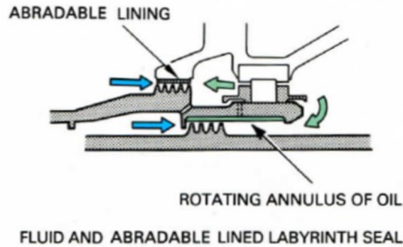
FLUID AND ABRADABLE LINED LABYRINTH SEAL
