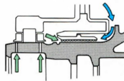
FLUID AND ABRADABLE LINED LABYRINTH SEAL
