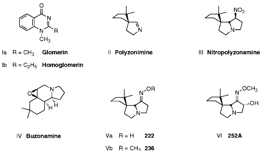
FIG. 1. Millipede alkaloids.
