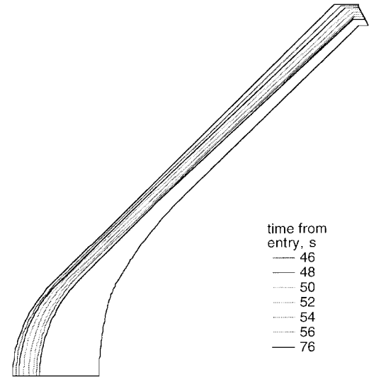
Fig. 13 Nominal heat shield shape history.
