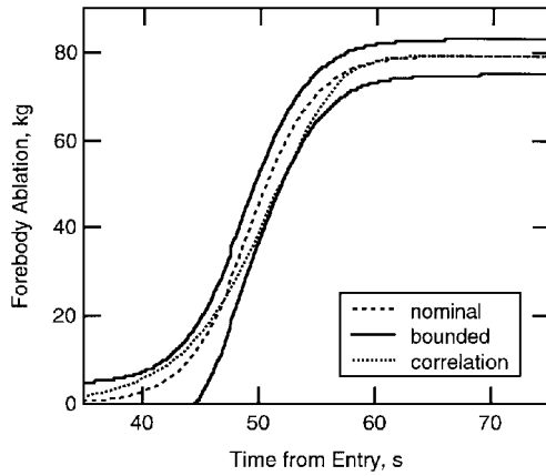
Fig. 14 Forebody ablative mass loss history.
