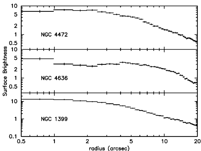
FIG. 2.— Chandra ACIS-S3 0.3\text{--}7 \text{ keV} central diffuse emission surface brightness distributions in units of \text{counts arcmin}^{-2} \text{ s}^{-1} . Annuli are centered on the X-ray centroids for NGC 1399 and NGC 4472 and on the near nuclear source for NGC 4636.
