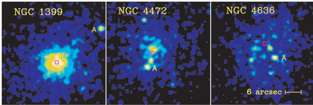
FIG. 1.— Chandra ACIS-S3 1.25–7 keV images of the central 50'' \times 50'' of NGC 1399, NGC 4472, and NGC 4636. The open, 1'' \times 1'' box indicates the position of the optical ( HST ) nucleus, the letter “A” represents the brightest point source. Relative shifts based on image registration have been applied for NGC 1399 ( 1''.5 ) and NGC 4636 ( 0''.9 ).
