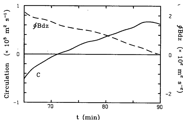
FIG. 12. The circulation and generation of circulation computed around the material curve shown in Fig. 11, vs time.
