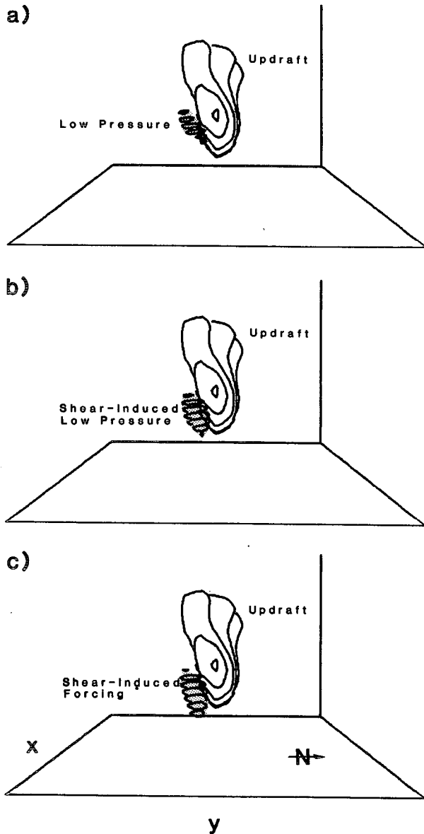
FIG. 16. A three-dimensional perspective (looking west) of the updraft ( >20 \text{ m s}^{-1} ) together with (a) perturbation pressure ( < -3.6 \text{ mb} ); (b) shear-induced pressure ( < -3.6 \text{ mb} ); and (c) forcing associated with the shear terms ( < -0.02 , units irrelevant) for the no-precipitation simulation at t = 150 \text{ min} on a 20 \times 20 \text{ km} portion of the computational domain. The vertical scale is exaggerated by a factor of 2.
