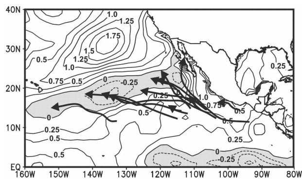
FIG. 3. SST departures from the 1968–96 long-term mean for the June–September 2004 period. Shaded areas denote cold anomalies and arrows mark the track of the 2004 named tropical cyclones.
