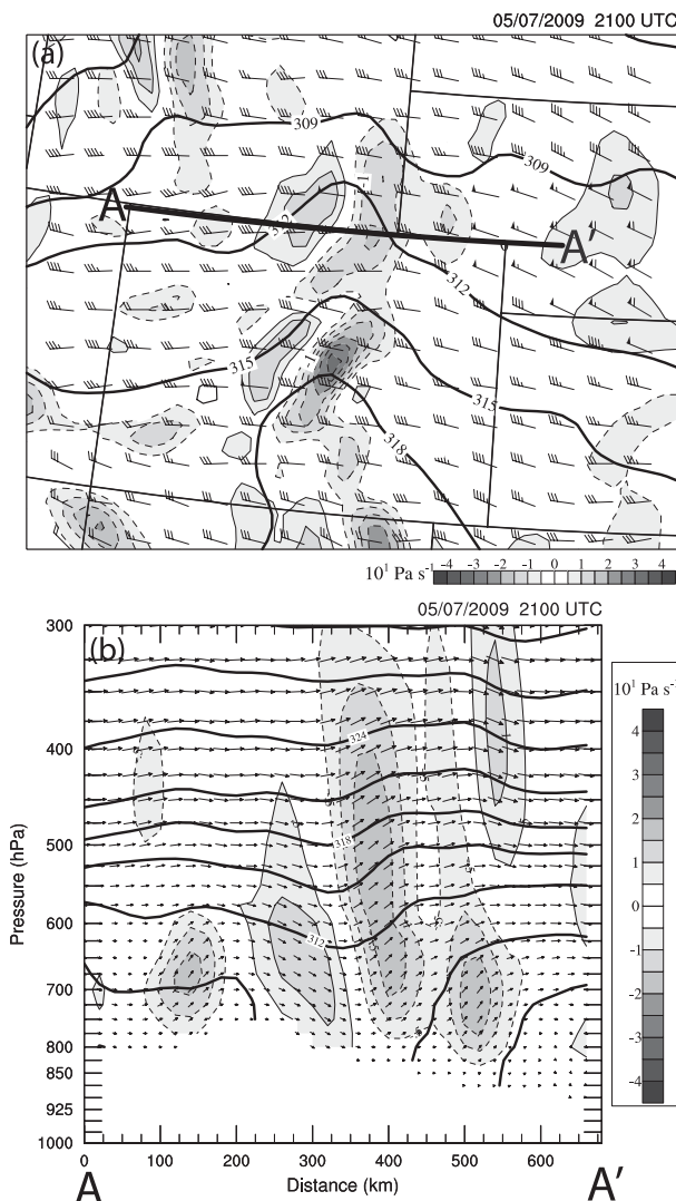
FIG. 7. (a) RUC analysis of 600-hPa pressure vertical velocity contoured and shaded every 0.5 \times 10^1 \text{ Pa s}^{-1} (negative values dashed) and potential temperature contours in thick black lines every 3 K valid 2100 UTC 7 May 2009. Half (full) wind bars are drawn every 2.5 (5) \text{m s}^{-1} and pennants represent 25 \text{m s}^{-1} . (b) As in (a), but for a vertical cross section along the line shown in (a) and with vectors illustrating the flow in the plane of the cross section.
