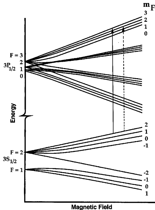
FIG. 6. Energy levels of Na in a magnetic field. The cycling transition used for laser cooling is shown as a solid arrow, and one of the nearly forbidden excitation channels leading to undesirable optical pumping is shown dashed.
