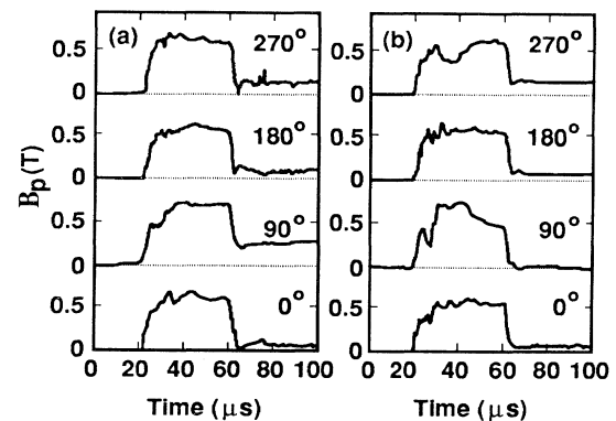
FIG. 2. (a) CT formation within the precompressor is usually stable and symmetric, as shown by the magnetic-field magnitude vs time at four azimuthal positions on the outer electrodes at z=0.12 m. (b) The early portion of CT formation is occasionally asymmetric but becomes symmetric within 30 \mu s. These data use hydrogen plasmas with the 10- \mu s-rise-time gun bank.
