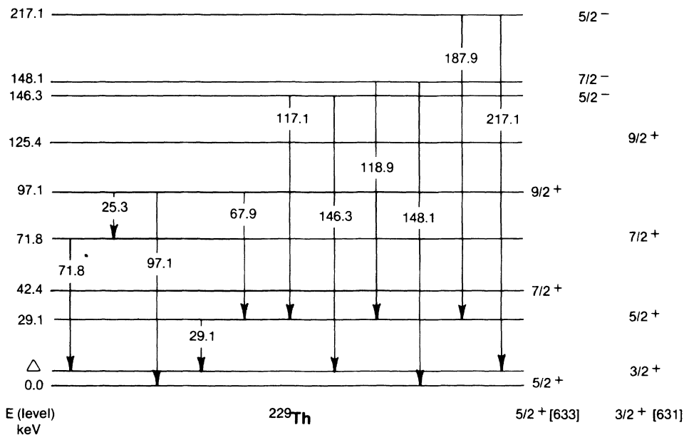
FIG. 1. Partial level scheme of ^{229}\text{Th} , showing those \gamma -ray transitions whose energy values were used in determining the energy separation \Delta of the \frac{3}{2}^+ [633] and \frac{3}{2}^+ [631] bandheads.
