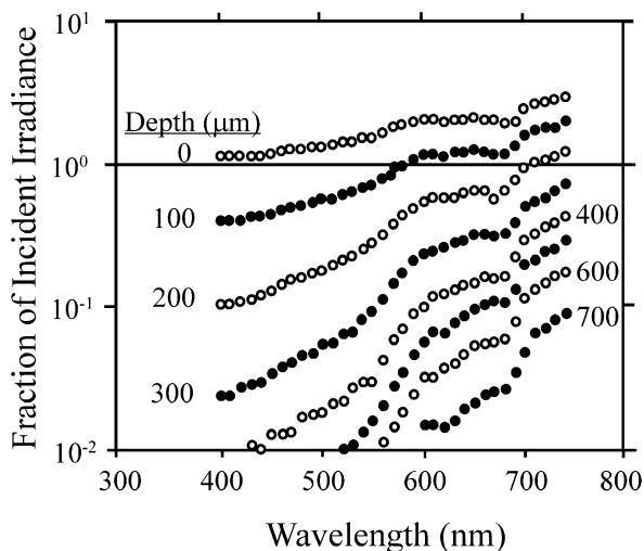
Fig. 2 Spectral attenuation: each spectrum shows the fraction of incident radiation in the soil at various depths (given in \mu\text{m} ). Filled and empty circles are alternated to aid in reading the figure (adapted from Garcia-Pichel and Belnap 1996)
