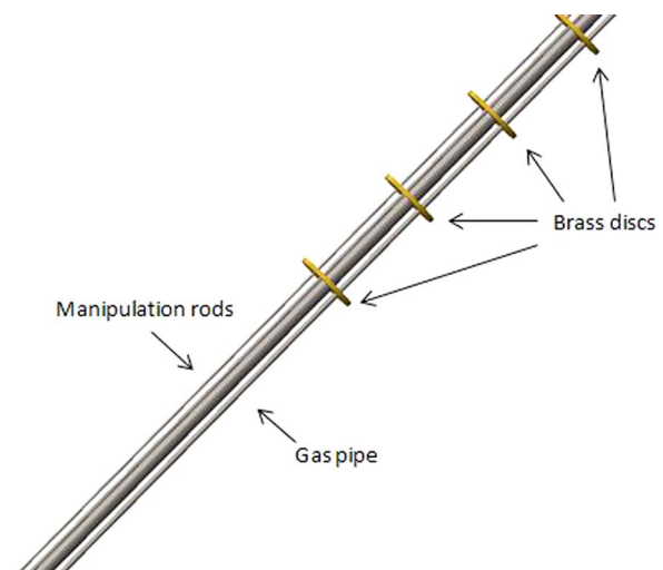
FIG. 2. CAD of shaft.
