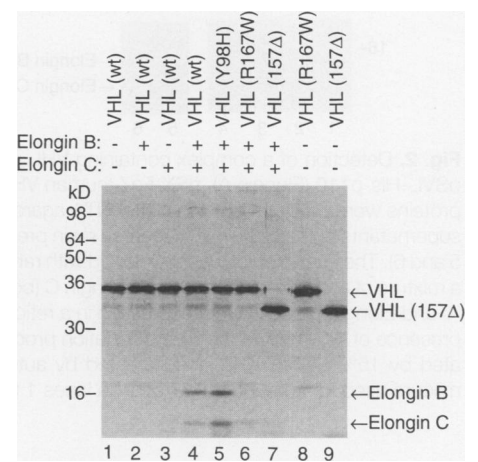
Fig. 5. Coimmunoprecipitation of Elongin B and C with wild-type (wt) or mutant VHL in vitro. The cDNAs encoding wild-type VHL (Fig. 7), mutant VHL (Y98H, 157Δ, R167W) (10), Elongin B, and Elongin C were expressed in a coupled transcription-translation system in the presence of 35 S-methionine. The translation products were immunoprecipitated with anti-Flag, fractionated by SDS-PAGE, and detected by autoradiography.
