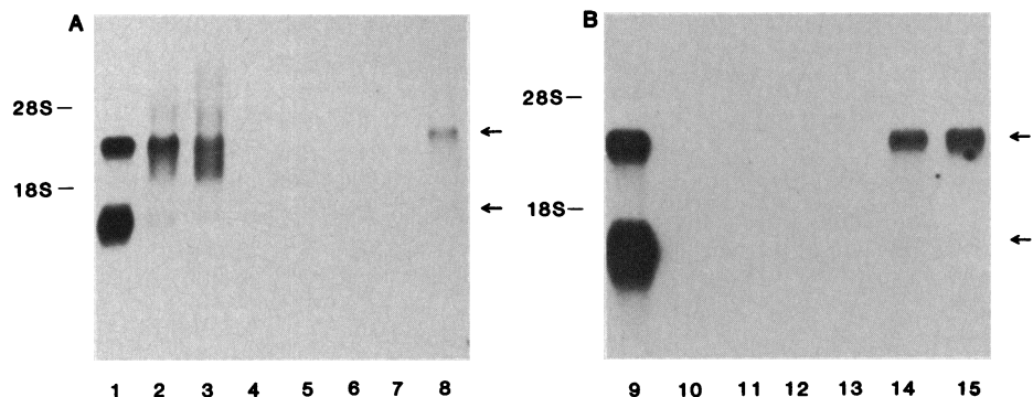
Fig. 2. Northern blotting analysis of tat-II induced IL-2 receptor mRNA expression. RNA was prepared from each cell line by the method of Chirgwin (31) and the poly(A) + fraction was enriched by oligo(dT) cellulose affinity chromatography (32). Ten micrograms of each RNA sample was size fractionated by formaldehyde-agarose gel electrophoresis and transferred to nitrocellulose filters (33). The filters were subsequently hybridized with 32 P-labeled IL-2 receptor cDNA radiolabeled by the random priming method of Feinberg and Vogelstein (34). Conditions of filter hybridization and washing were as previously described (15). Similar results were obtained with four independent preparations of RNA. Cell lines: 1 and 9, HUT 102B2; 2 and 15, Jurkat- tat-II -7; 3 and 14, Jurkat- tat-II -6; 4, Jurkat-anti- tat-II -16-4; 5, Jurkat-anti- tat-II -16-3; 6, Jurkat-anti- tat-II -16-1; 7 and 13, nontransfected Jurkat; 8, Jurkat induced with PHA and PMA; 10, Raji-anti- tat-II -16-1; 11, Raji- tat-II -21-2; 12, Raji- tat-II -21-3.
