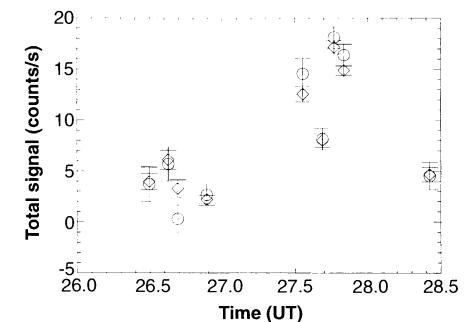
Fig. 5. X-ray and EUV cometary light curves for Hyakutake taken on UT 26 to 28 March 1996. All error bars are \pm 2\sigma . s: HRI, 0.1 to 2.0 keV light curve (open diamonds). WFC .09 to .20 keV light curve (open circles) scaled by a factor of 32.
