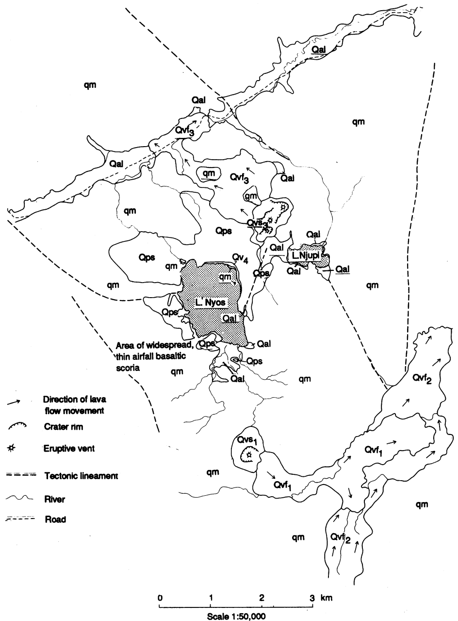
Fig. 2. Photoreconnaissance geologic sketch map of Lake Nyos. Abbreviations: Qal, alluvium; Qvs 1 , basaltic scoria southeast of Lake Nyos; Qvf 1 , basaltic flow southeast of Lake Nyos (source south of map edge); Qvs 3 , basaltic scoria northeast of Lake Nyos; Qvf 3 , basaltic flow northeast of Lake Nyos; Qps, phreatomagmatic pyroclastic surge deposits surrounding Lake Nyos; Qv 4 , basaltic scoria and flow along northeast shore of Lake Nyos; and qm, coarse-grained biotite quartz monzonite of pre-Tertiary age (overlain by lateritic soil).
