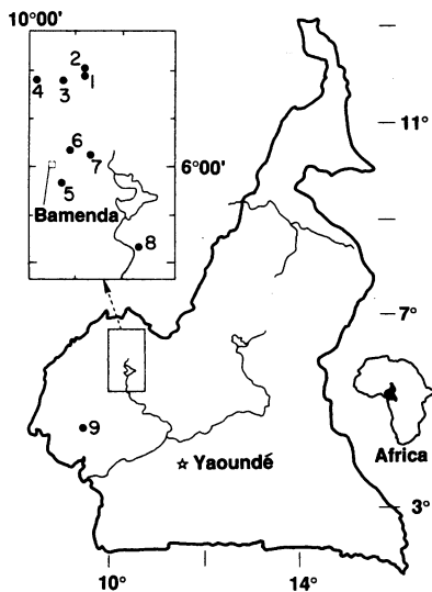
Fig. 1. Location of Cameroon and northwestern lakes. Labeled sites: 1, Lake Nyos; 2, Nyos spring; 3, Lake Nyi; 4, Lake Wum; 5, Lake Bambuluwe; 6, Lüh spring; 7, Gesel spring; 8, Lake Monoun; and 9, Barombi Mbo.
