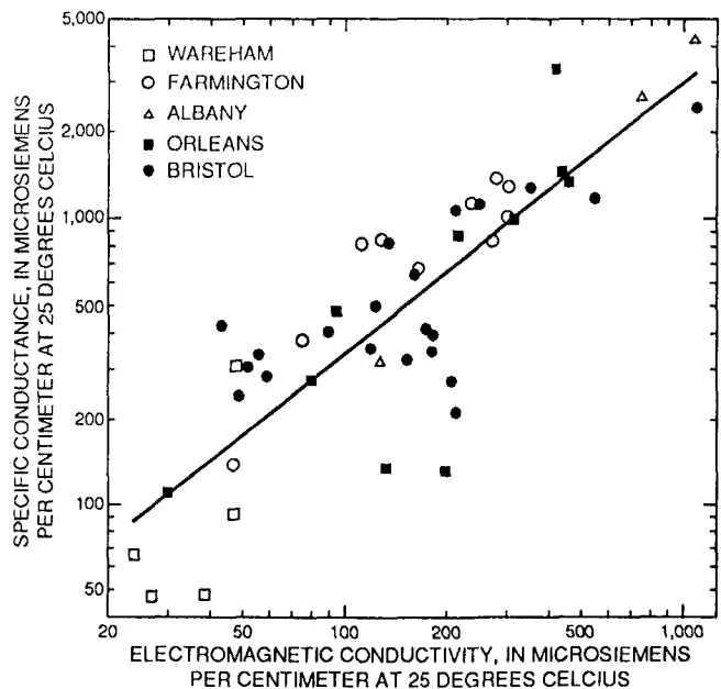
Figure 8. Relation between electromagnetic conductivity and specific conductance of the water from selected well screen intervals in glacial sand-and-gravel aquifers.
