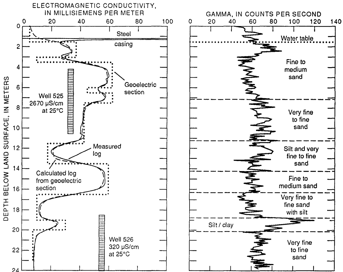
Figure 7. Electromagnetic, gamma, and lithologic logs; specific conductance data; and geoelectric section for the pair of wells 525 and 526 at the Albany landfill site.
