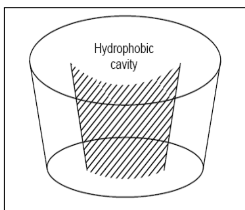
Figure 1.3: Physical shape of the CD molecule (Wei-Qin and Hong, 2008)
