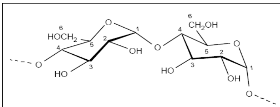
Figure 1.2: Conformation and numbering of the CDs (Wei-Qin and Hong, 2008)
