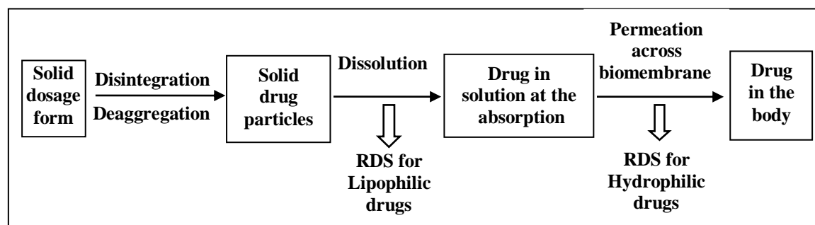
Figure 1.1: Two rate determining steps (RDS) in the absorption of drugs from orally administered formulations.
