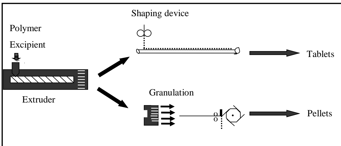
Figure 1.5: Scheme of hot melt extruder (Leuner and Dressman, 2000)
