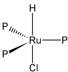
axial,trans
