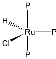
equatorial
