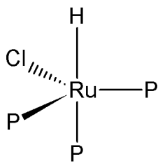
axial-(H),cis
