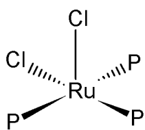
apical
