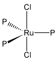
axial,trans
