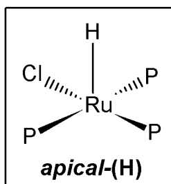
axial,trans
