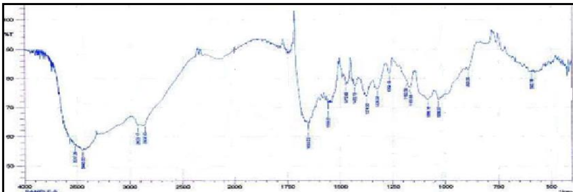
Fig.2: FTIR spectra of Lamivudine, Sodium alginate, Chitosan and SS-5
