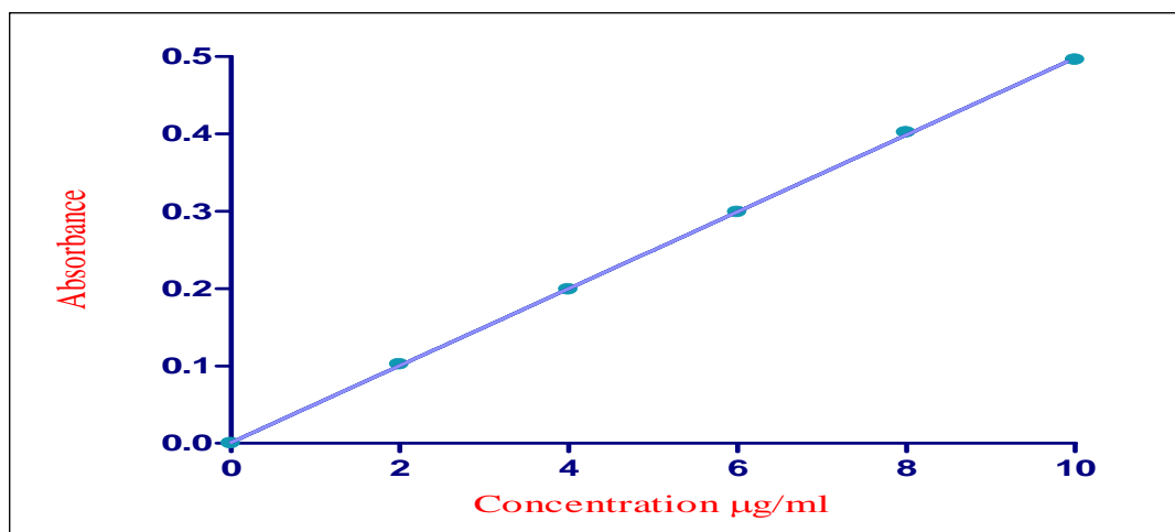
Fig. 1: Calibration curve for lamivudine in pH 7.4 phosphate buffer
