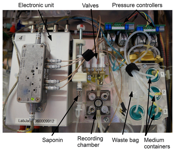
Fig. 2. OoClamp system. Schematic illustration (left) and photograph (right) of the OoClamp system. The media exchange was driven by air pressure. The medium containers were pressurized with a pressure controller, such that the medium was pressed out through capillaries and into the recording chambers. Valves before the recording chamber allowed the medium flow to be controlled. The used medium was collected in a waste bag. Gentle pressure was applied to the upper compartment to ensure good electrical isolation of the membrane patch. The OoClamp was controlled via USB with an external laptop. Saponin solution was injected with 2-ml syringes into the upper compartment of the recording chamber after the oocyte was placed and the top pressure was applied (not shown in the left illustration). Approximately 120 \mu l of Saponin was injected by slowly turning a thread.
