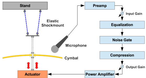
Figure 2: Simplified system layout.
