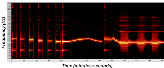
Figure 3: Spectrogram of varying pitch between latching strikes (left) and continuously (center) with a 12-inch china splash. Amplitude modulation displaying sidebands can be seen on the right.
