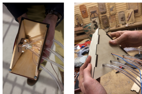
Figure 8: The inside and back of the siren disk stand.
