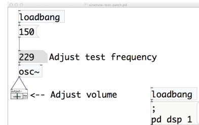
Figure 4: Pd patch for searching for resonance frequencies contributing to rattling.
