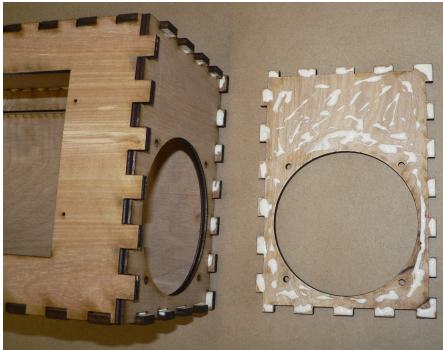
Figure 3: The thickness of faces containing loudspeaker drivers can be doubled simply by gluing two layers of laser-cut plywood together.
