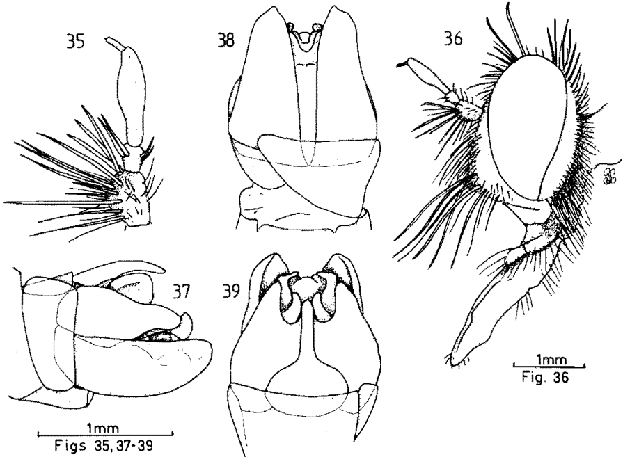
Figs 35-39. Remotomyia albosetatus (Hull). 35-36. Bagani female. 35. Antenna, lateral aspect. 36. Head. 37-39. Oshikango male genitalia. 37. Lateral. 38. Ventral. 39. Dorsal.
