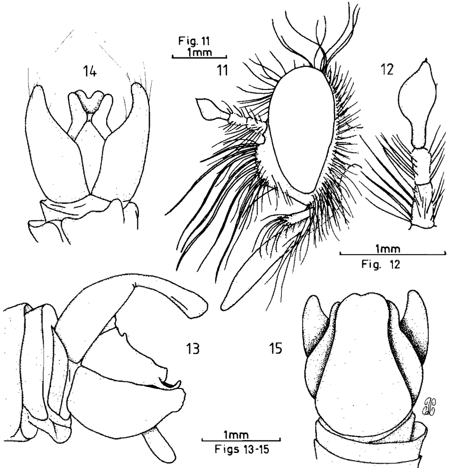
Figs 11-15. Daspletis hirtus Ricardo. 11-12. Kalahari Gemsbok Park male. 11. Head. 12. Antenna, lateral aspect. 13-15. Sawmills totype male genitalia. 13. Lateral. 14. Ventral. 14. Dorsal.
