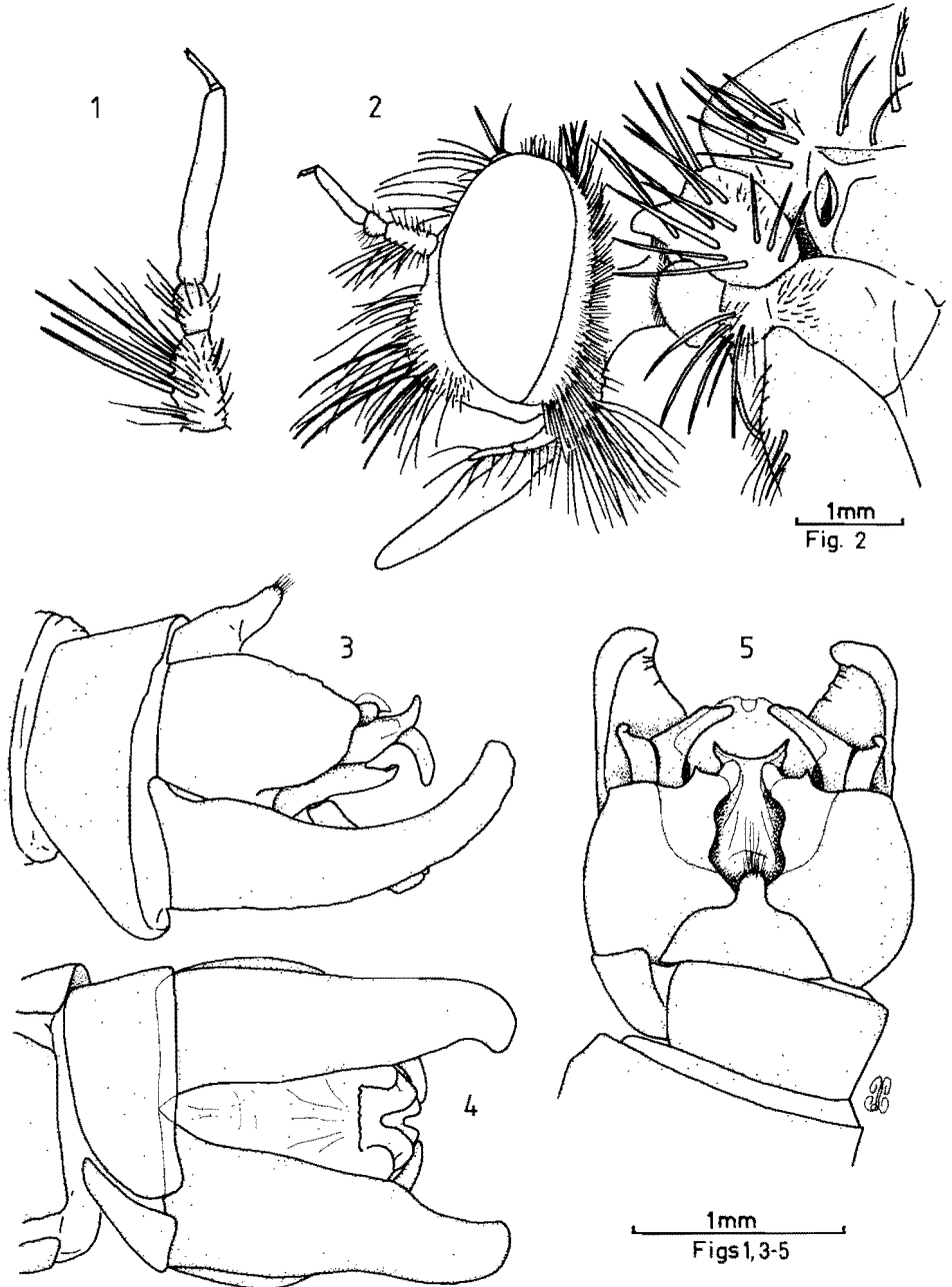
Figs 1-5. Anasillomos chrysopos spec. nov. paratype male. 1. Antenna, lateral aspect. 2. Head and part of thorax. 3-5. Genitalia. 3. Lateral. 4. Ventral. 5. Dorsal.
