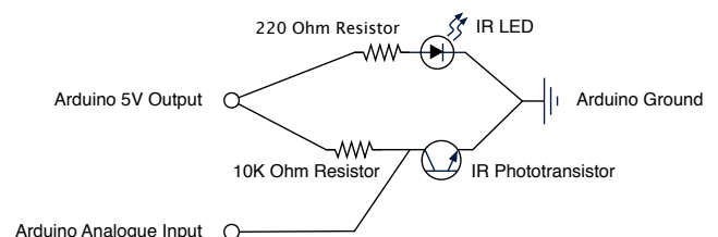
Figure 4: Circuit for the heartbeat sensor.
