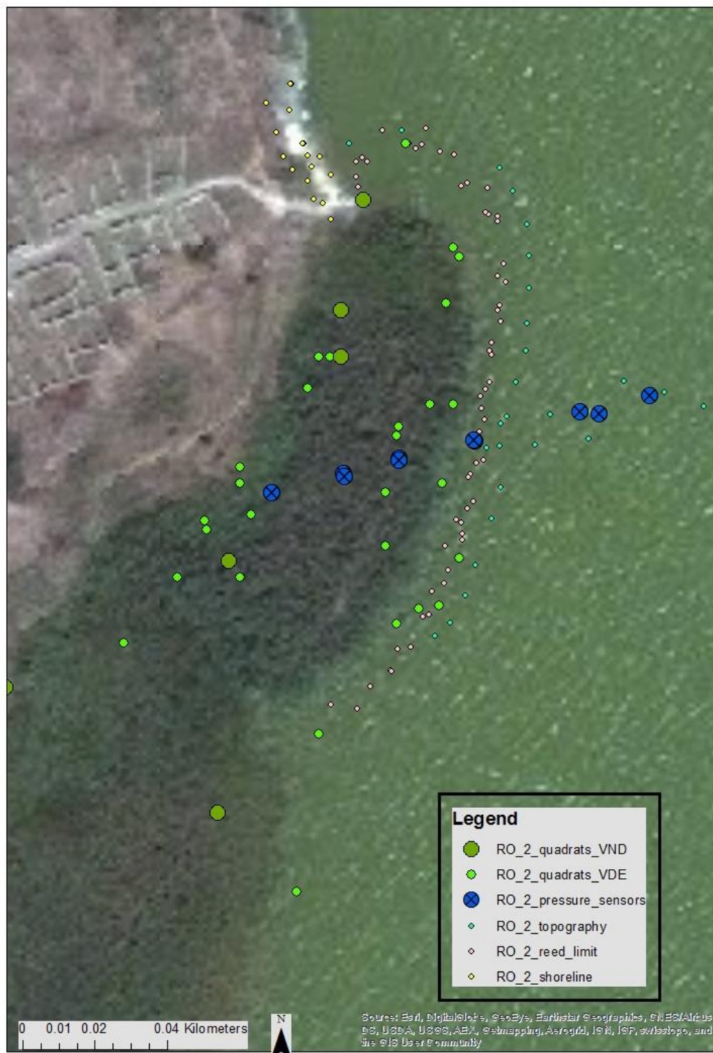
Figure 6 Locations of topographic surveys, monitoring equipment and sampling quadrats deployed at RO Y2 site
