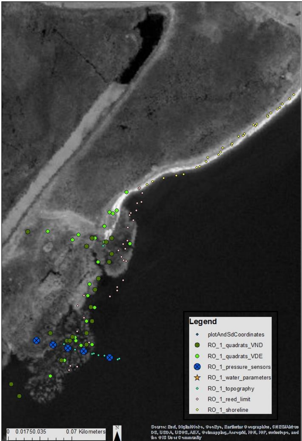
Figure 7 Locations of topographic surveys, monitoring equipment and sampling quadrats deployed at RO Y1 site
