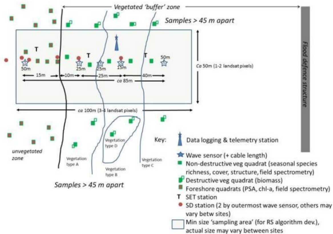
Figure 3 Schematic illustration of field sample layout used within the FAST project. Individual site locations vary from this and geo-referenced information of each sensor location is provided to accompany the wave measurement data uploaded on the FAST data repository.
