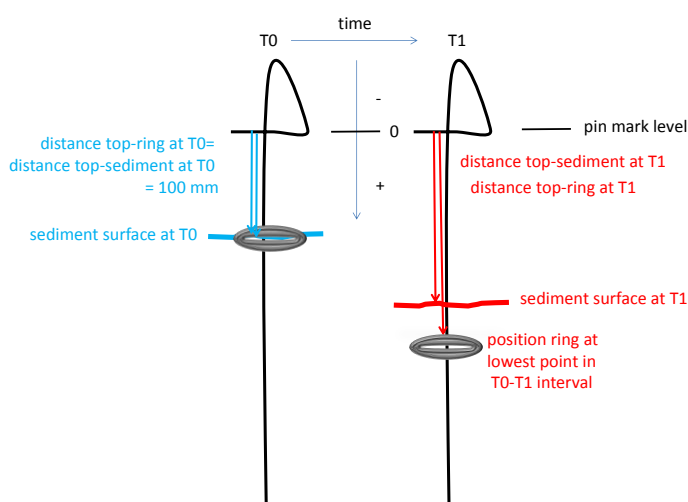
Figure 17 Example of an erosion pin (drawn in black) with readings at T0 and T1. Both distance top-ring and distance top-sediment are measured at each date. Note the sign of the distance measurement (positive towards ring). From the differences at T0 and T1, maximal erosion and net deposition/erosion is calculated.
