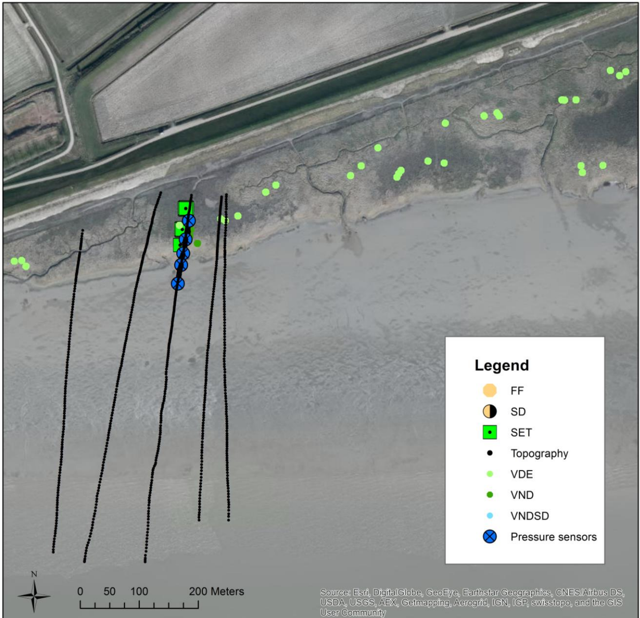
Figure 11 Locations of topographic surveys, monitoring equipment and sampling quadrats deployed at NL Y2 site
