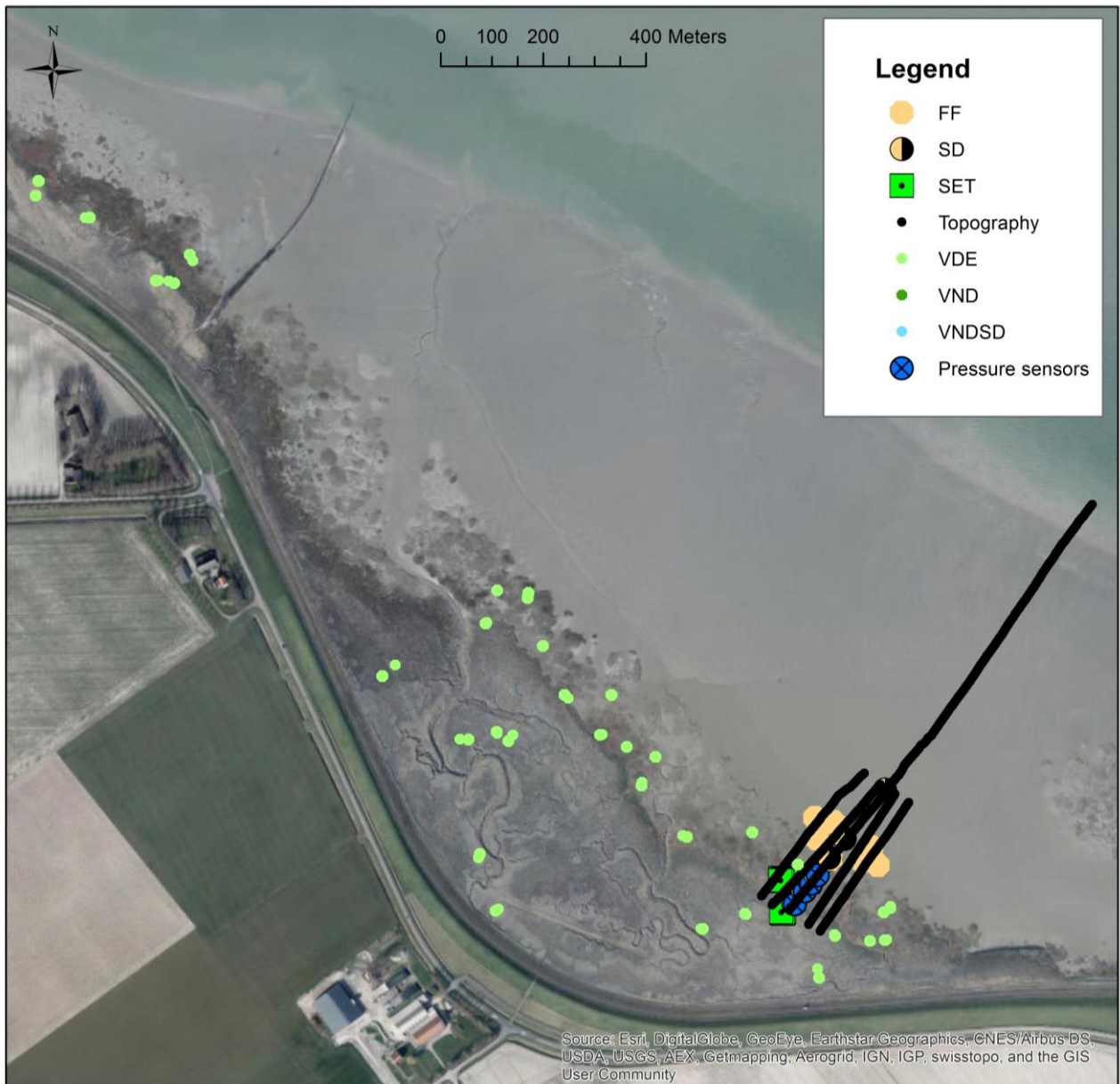
Figure 10 Locations of topographic surveys, monitoring equipment and sampling quadrats deployed at NL Y1 site
