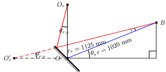
Fig. 6. The introduction of BSs extends the optical path from the centre of the sample at O_r to the detector at B . The scatter direction relative to the mirror image of O_r' is calculated from the direction relative to the centre of the detector rotation O .
