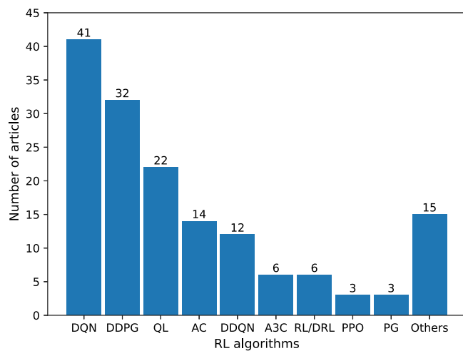
Fig. 7. Distribution of different RL techniques of the proposed solutions.
