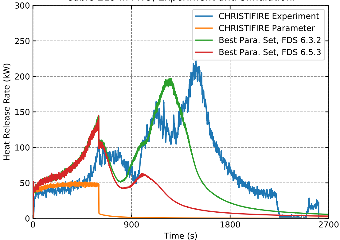
Cable 219 in MT3, Experiment and Simulation.
