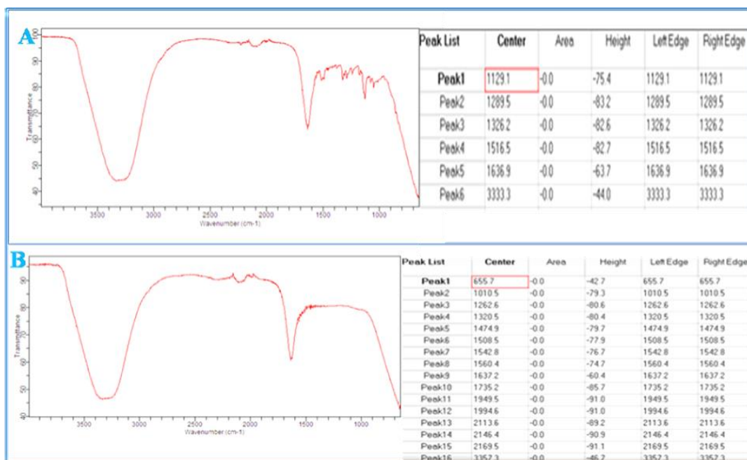
Fig. 3: FT-IR spectral image of various functional groups (1000 to 3500 cm -1 ) A- A. aspera aqueous extract and B- Aqueous extract-based synthesized AgNPs
