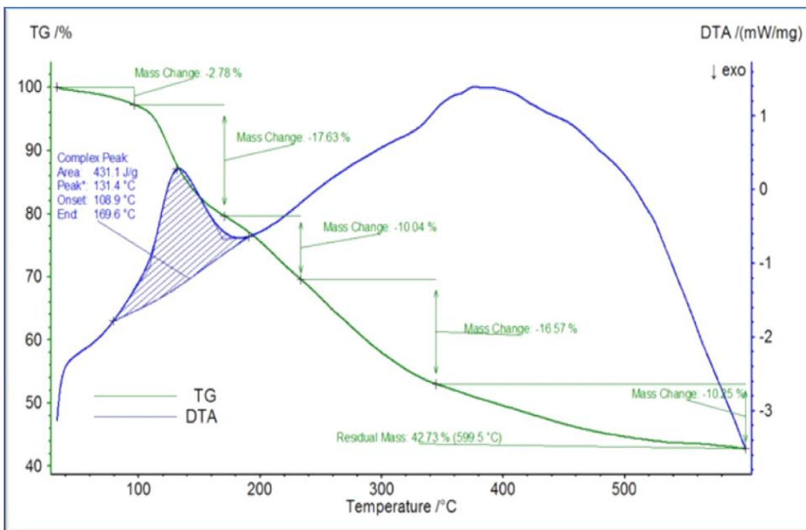
Fig. 7: TG-DTA analysis of A. aspera mediated AgNPs
