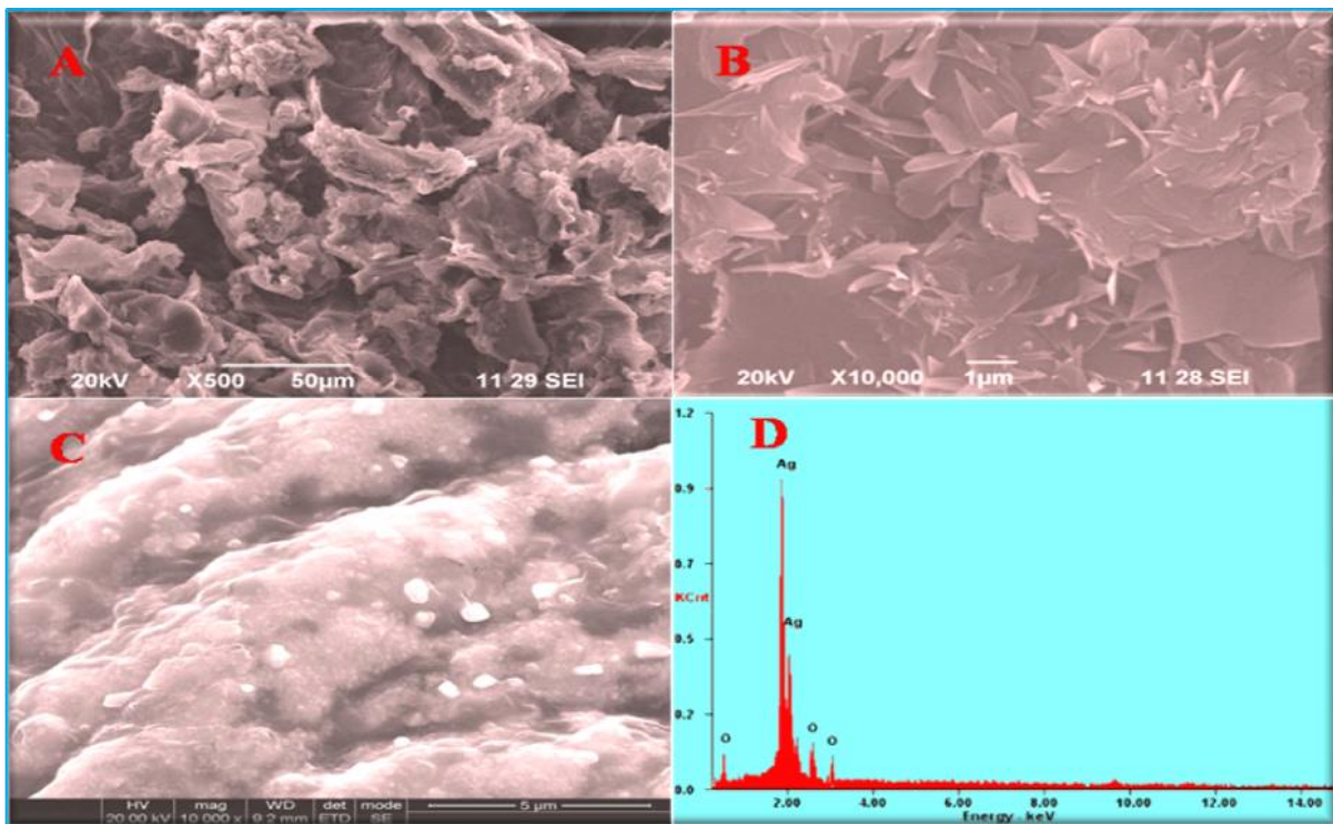
Fig. 5: A. SEM micrograph of A. aspera aqueous extract, B. SEM micrograph of 1 mM silver nitrate solution, C. SEM micrograph of A. aspera aqueous extract-based synthesized AgNPs and D. EDX analysis of AgNPs synthesized from the aqueous extract of A. aspera
