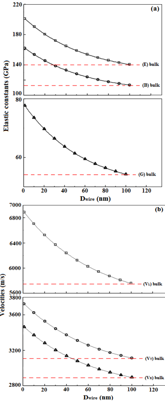
Fig. 3 Effects of ZnO wire diameters ( D_{wire} ) on (a) elastic constants: E ( \square ), B ( \circ ) and G ( \Delta ) and (b) velocities: V_L ( \square ), V_T ( \circ ) and V_R ( \Delta ). The horizontal dashed lines represent the corresponding calculated bulk value along the [0001] direction
