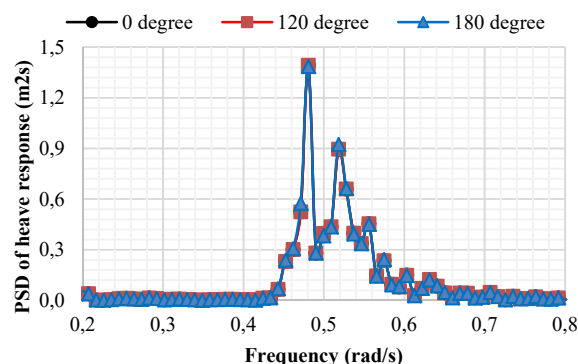
(c) Heave Response
