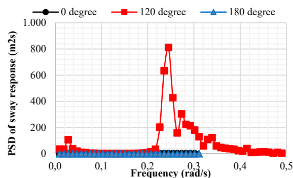
(b) Sway Response
