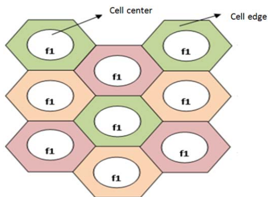
Fig. 6 Soft Frequency Reuse
