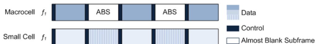
Fig. 8 Time-domain technique based on ABS concept [9]
