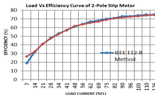
Fig. 8 Comparison of the Performance on 5 HP Motor
