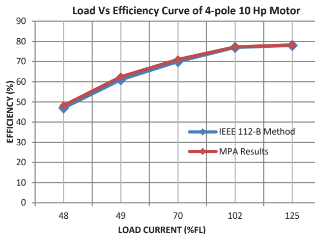
Fig. 10 Comparison of the Performance on 10 HP Motor
