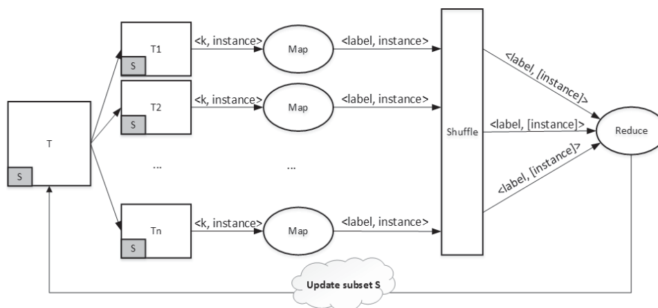
Fig. 3 Flowchart of FCNN-MR algorithm
