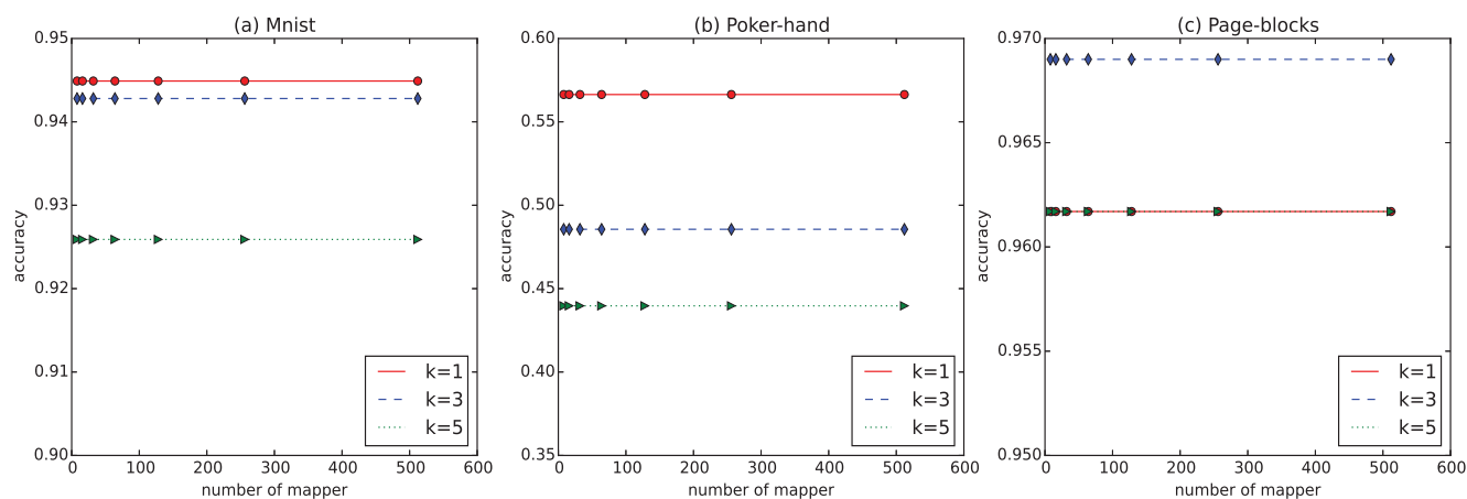
Fig. 4 The accuracy with different number of mapper
