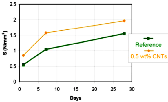
Fig. 3 Dissipated Energy Density vs. days of curing [7]
