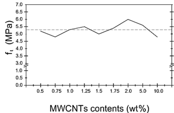
Fig. 2 Tensile strength of mortar cylinders cured for 7 days against CNT content (dashed line: samples without CNTs) [7]
