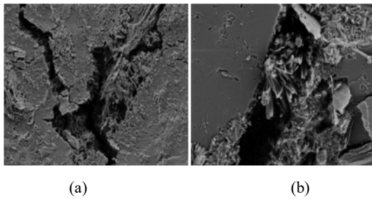
Fig. 4 Microstructure of concrete after frost resistance test: (a) No CNTs (reference sample with frost resistance of F200), (b) CNT-reinforced sample (F400) [5]
