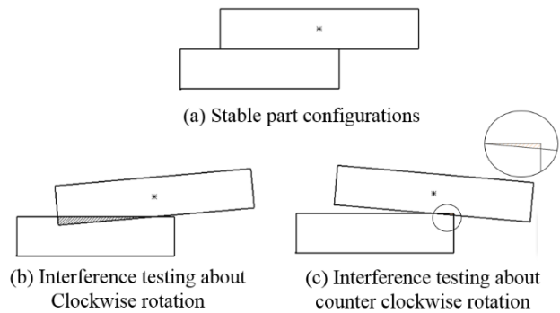
Fig. 7 Partially stable assembly sets
