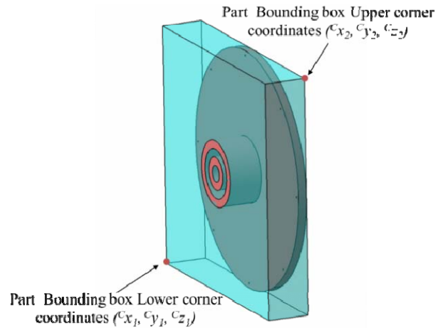
Fig. 3 Part-C Bounding box representation
