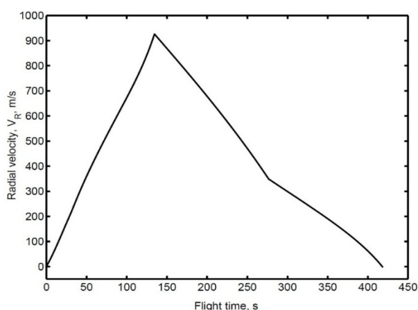
Fig. 7 Radial velocity variation over Zenit-2 flight time
