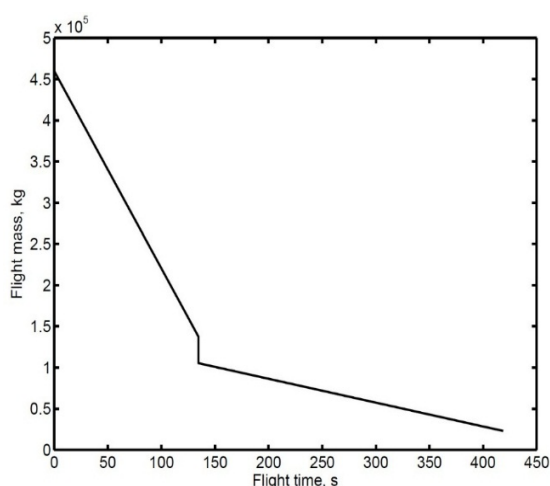
Fig. 13 LV in flight mass drop during flight
