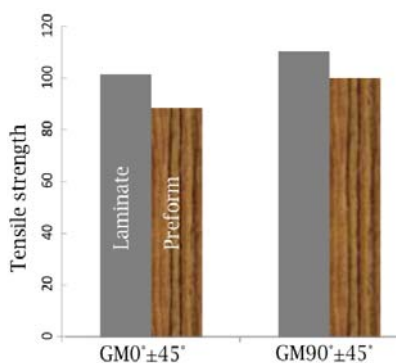
Fig. 8 Tensile Strength of Glass Preforms and Laminate
