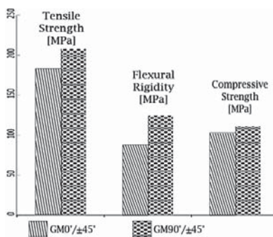
Fig. 9 Comparative Properties of Laminates
