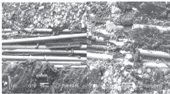
(b) Preform Structure in Laminate
