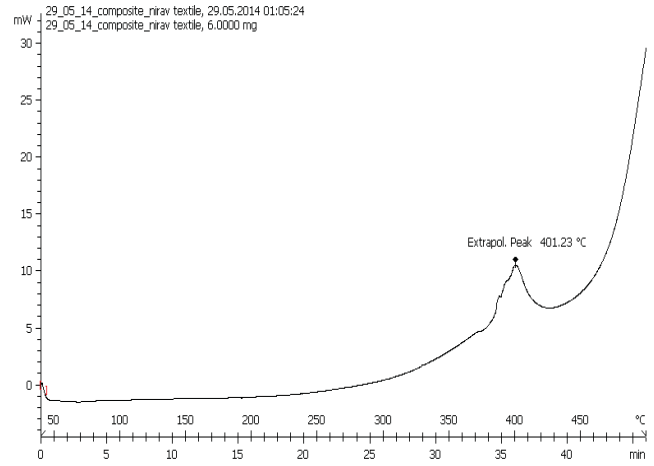
Fig. 6 DSC Analysis of Glass Laminate (GM0°/±45°)
