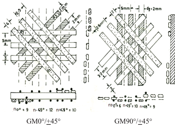
(a) Preform Structure
