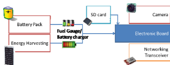
Fig. 3 Architecture of the smart camera
