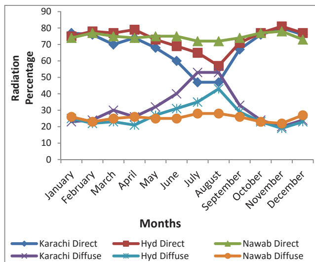
Fig. 9 The pattern of variation of direct and diffuse solar radiation for three cities of Sindh
