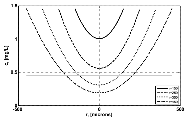
Fig. 4 Simulation results of dissolved oxygen concentration inside of the various-radius cell aggregates ( C_M= 3 \text{ mg/L} ). Solid gray line marks border ( c < 0.45 \text{ mg/L} ) where strong oxygen limitation inside of the cell aggregates occurs
