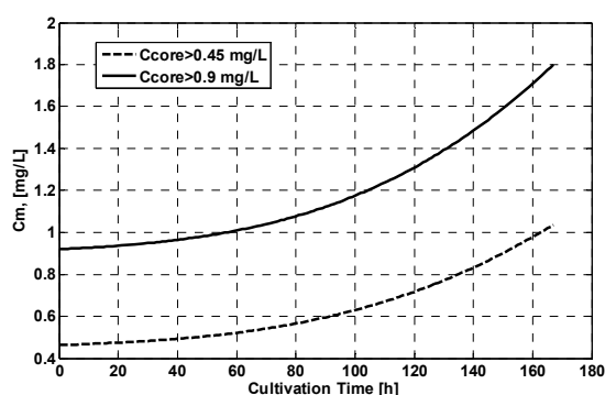
Fig. 5 Rational profiles of dissolved oxygen concentration C_{M\_min}(t) in stem cells cultivation process
