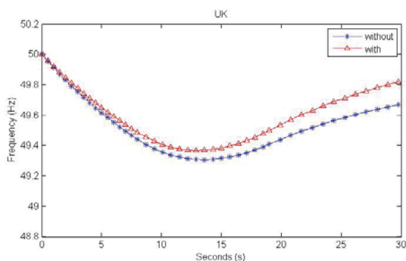
Fig. 12 Primary Frequency Response for the UK
