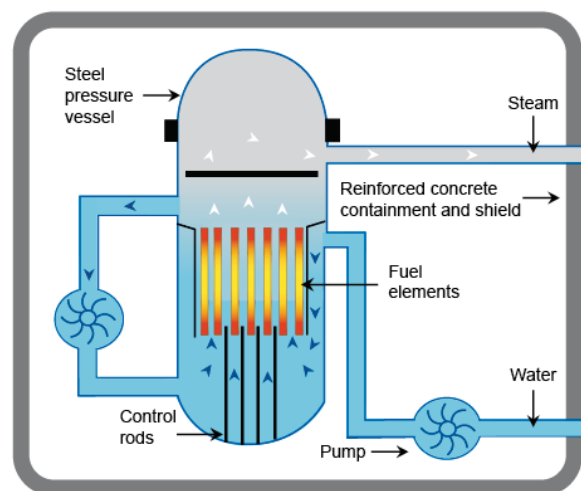
Fig. 2 Boiling Water Reactor [2]
