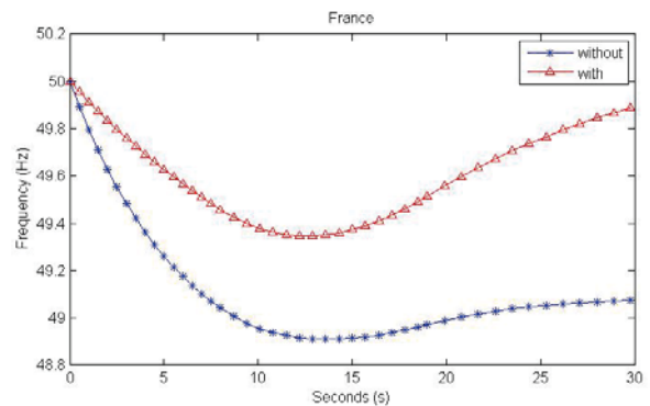
Fig. 10 Primary Frequency Response for France
