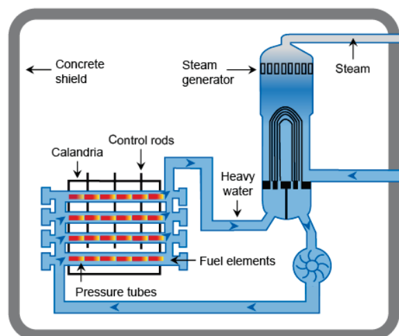
Fig. 4 CANDU Reactor [2]
