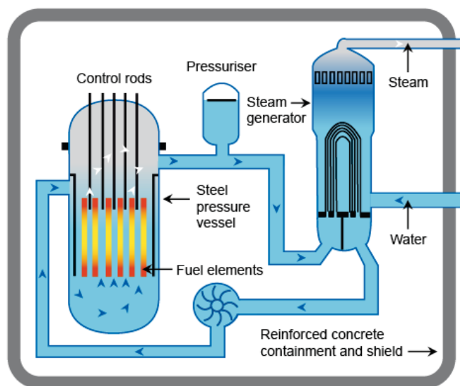
Fig. 1 Pressurised Water Reactor [2]
