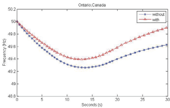
Fig. 8 Primary Frequency Response for Ontario, Canada
