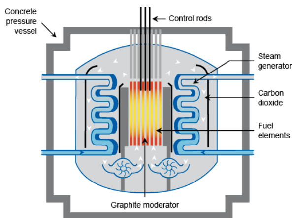
Fig. 3 Advanced Gas-Cooled Reactor [2]
