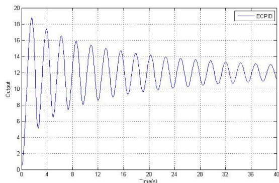
Fig. 13 Step response for input with amplitude 7 (ECPID)
