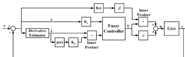
Fig. 1 Closed-loop control structure for parameter adaptive PID-type FLC via function tuner [19]
