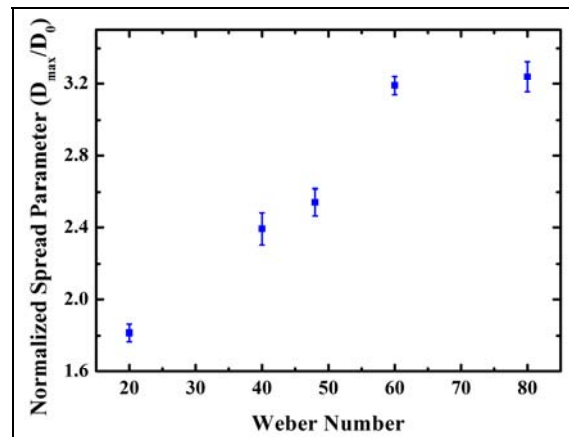
Fig. 9 Normalized spread parameter ( D_{max}/D_0 )
