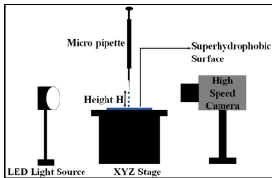
Fig. 3 High speed imaging setup for drop impact study
