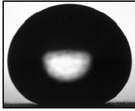
Fig. 4 Water droplet on superhydrophobic paper surface
