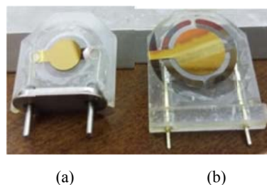
Fig. 2 Image of the version V1.0 methacrylate holder (a) ICM \frac{1}{2} " sensor (b) INFICON 1" sensor
